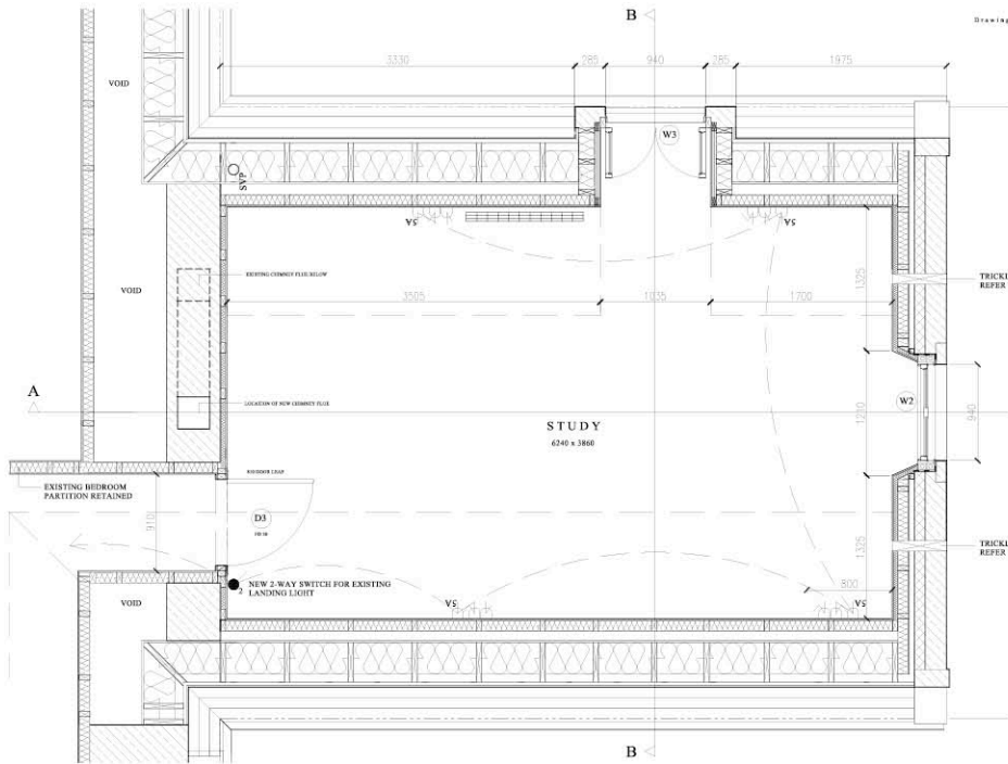
Detail construction plan of study/bedroom.
